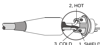
Illustration 2.1: Balanced connection of input
