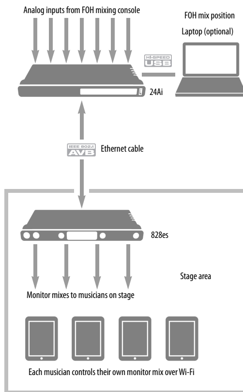
Figure 6-4: An example of using the AVB Expansion preset: 24 channels from the FOH console are being distributed to musicians on stage as 4 separate monitor mixes.
