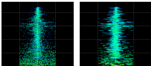
Figure 10-21: The same Phase Analysis displayed in Line versus Scatter mode.
