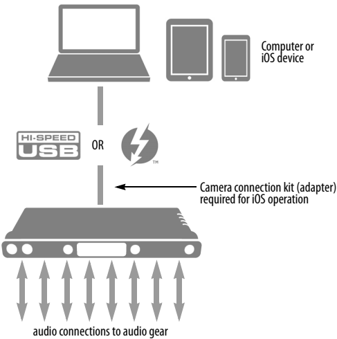
Figure 6-1: Using the 828es as an audio interface.
